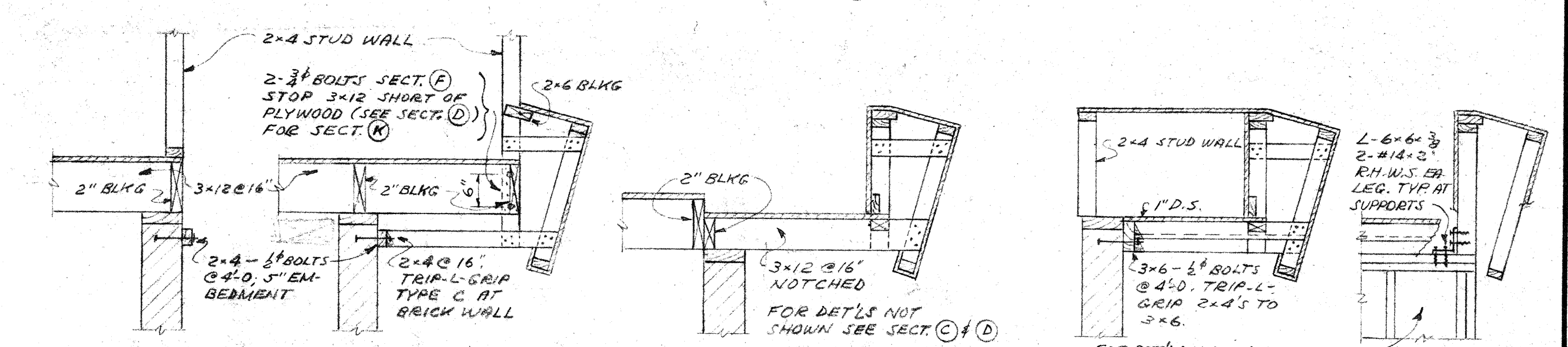
SECTION E SCALE: 1/2"=1'-0" SECTION F AS SHOWN SECTION G SCALE: 1/2"=1'-0" SECTION H SCALE: 1/2"=1'-0" SECTION J SCALE: 1/2"=1'-0"
