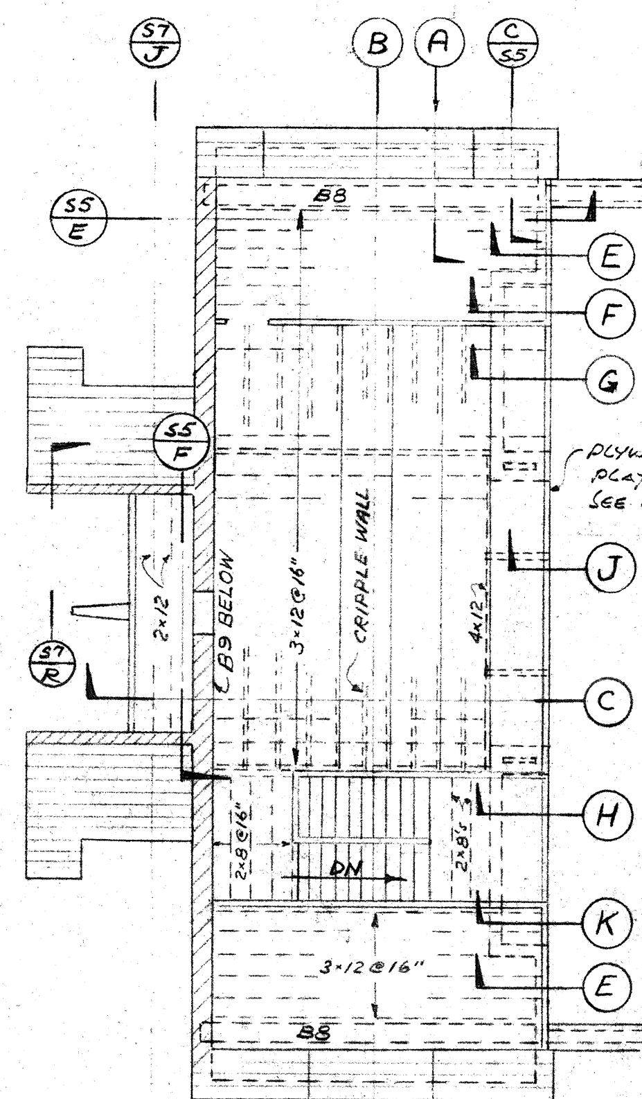
BALCONY FRAMING PLAN SCALE: 3/8"=1'-0"
